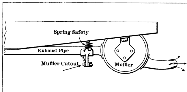
Fig. 67—Side view, showing muffler to rear of chassis, and muffler cut-out located so far back that exhaust will not float up into the car
